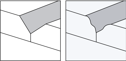
MAXIBEVEL
